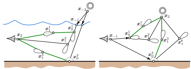
Figure 3: Left: Classic light tracing with next event estimation or equiangular sampling samples a direction at a volume vertex x_0 or surface vertex x_0^3 towards x_1^1 and x_1^3 , respectively, typically by importance sampling the BSDF. The high throughput 2-segment connections (green) that bend at these vertices toward the eye and create an intermediate vertex x_1^1 or x_1^3 are sampled with low probability and thus suffer from variance. Our technique is tailored to sample these connections efficiently. Right: The path tracing case analogously samples such 2-segment connections towards the light.
