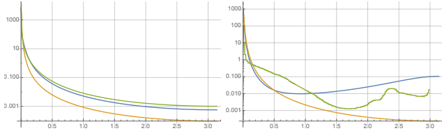
Figure 9: Fournier-Forand (left) and Mie (right) phase functions fitted to a single Henyey-Greenstein (orange) and a two-term Henyey-Greenstein (blue) phase function [GSM08]. For the single, g = 0.99527 resp. g = 0.988264 ; the double has g_1 = 0.997229 and g_2 = 0.959952 with a weight of 0.339242 and g_1 = 0.990344 and g_2 = -0.439579 with a weight of 0.712146 . The green line is the ground truth phase function. A good summary of existing analytical phase functions can be found in [Sha15].
