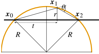
Figure 5: The geometry of the three path vertices x_0, x_1, x_2 and the angle \theta between the two segments, sampled according to the phase function f_s(x_1) . The arc radius R , the polar coordinate r and the fractional distance t assume the path geometry has been normalised such that \bar{x}_0\bar{x}_2 = 1 .
